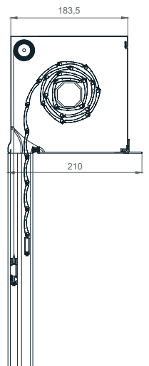
CONCEALED 90° 180
