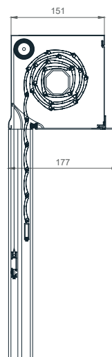
CONCEALED 90° 150
