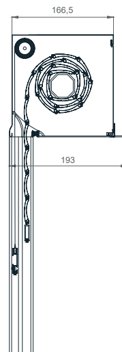
CONCEALED 90° 165
